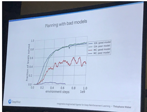
Figure 2: Even with a bad model the approach seems to work well.
